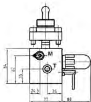
Positioning Cetop size 3 for clack electro-valve
