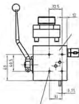
Positioning Cetop size 3 for clack electro-valve
