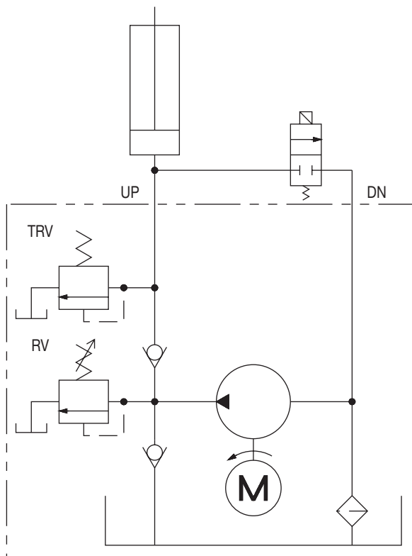
"WW" CIRCUIT
